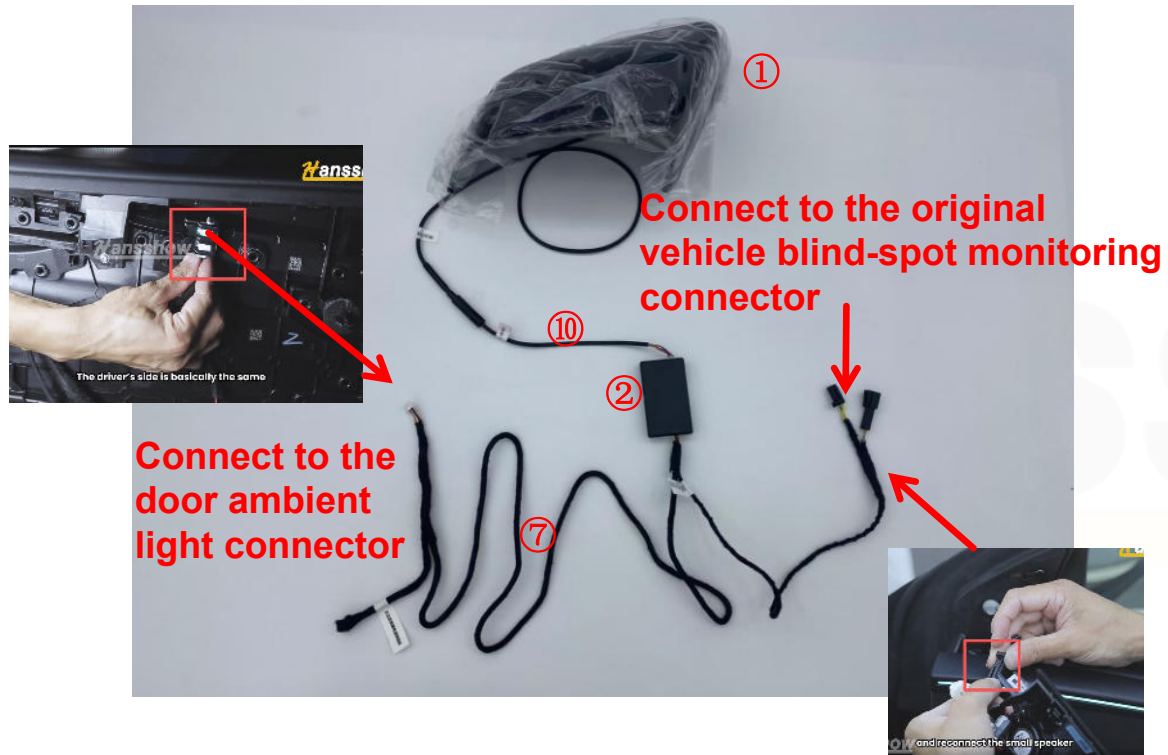
Left-Side Wiring Diagram
