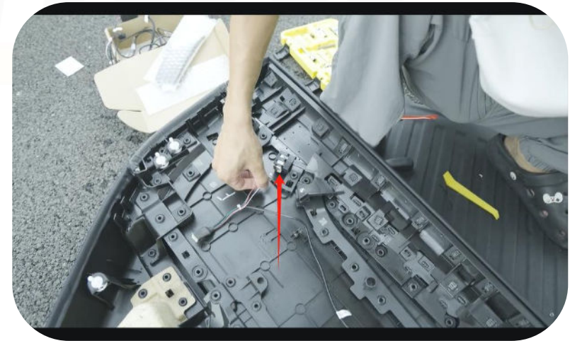
9. Connect the power cable to the ambient light port.
