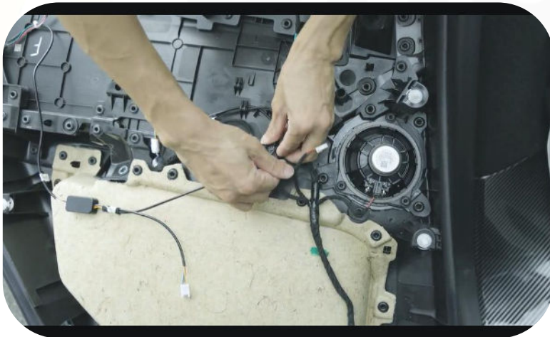
12. Reconnect original door panel cables.
