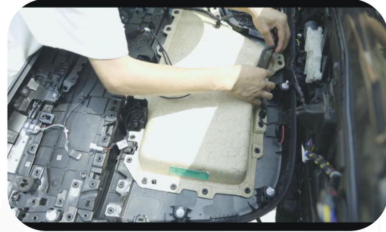
16. Reconnect all wiring to the door panel.
